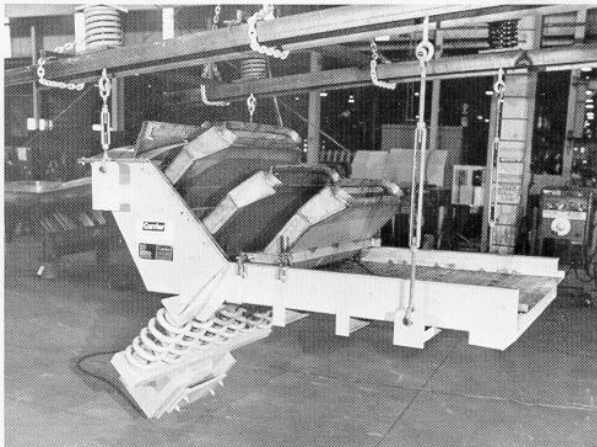
Feeder/screener for nylon pellets. Vacuum for angel hair pickup and removal.
